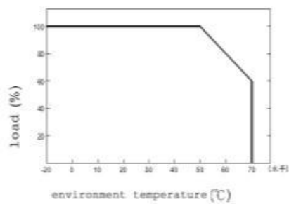
Derating Curve
